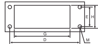
Panel Cutout
